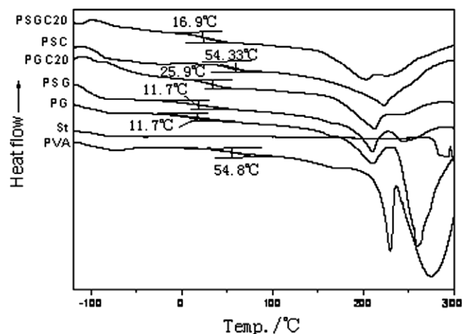
Fig. 3. The effects of glycerol and CA on DSC curve of PVA and PVA/starch blends.
